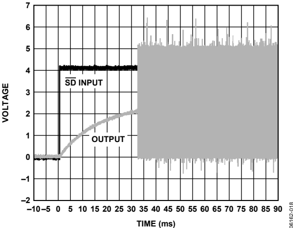
Figure 35. Turn-On Response
