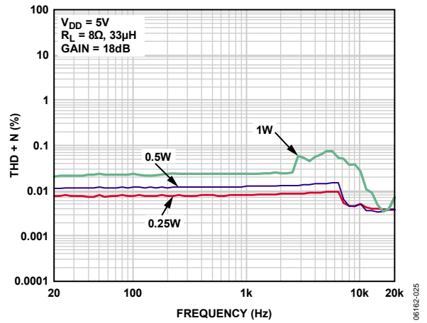
Figure 13. THD + N vs. Frequency, V_{DD} = 5\text{ V} , R_L = 8\ \Omega , A_V = 18\text{ dB}
