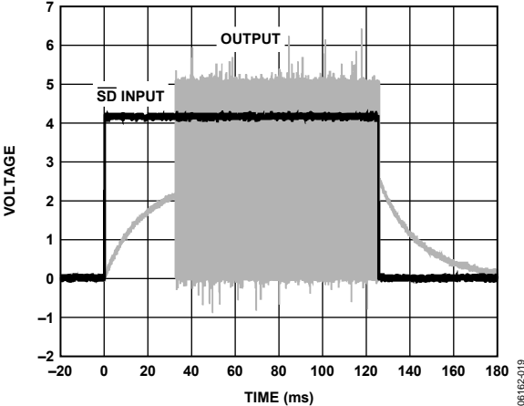
Figure 36. Turn-Off Response
